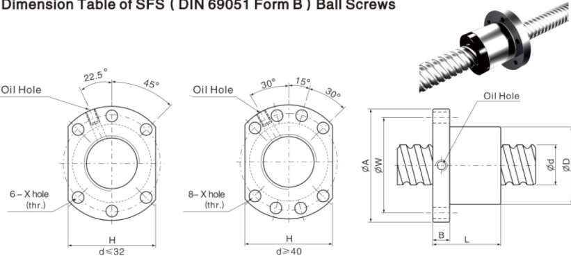
Dimension Table of SFS ( DIN 69051 Form B ) Ball Screws
